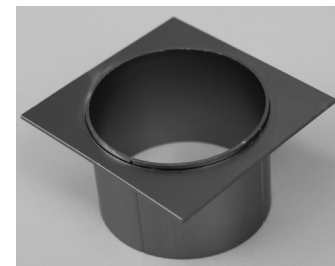
Infinity Channel Drain Waste Outlet 60mm Flange / 50mm Waste Outlet Gun Metal Brushed
