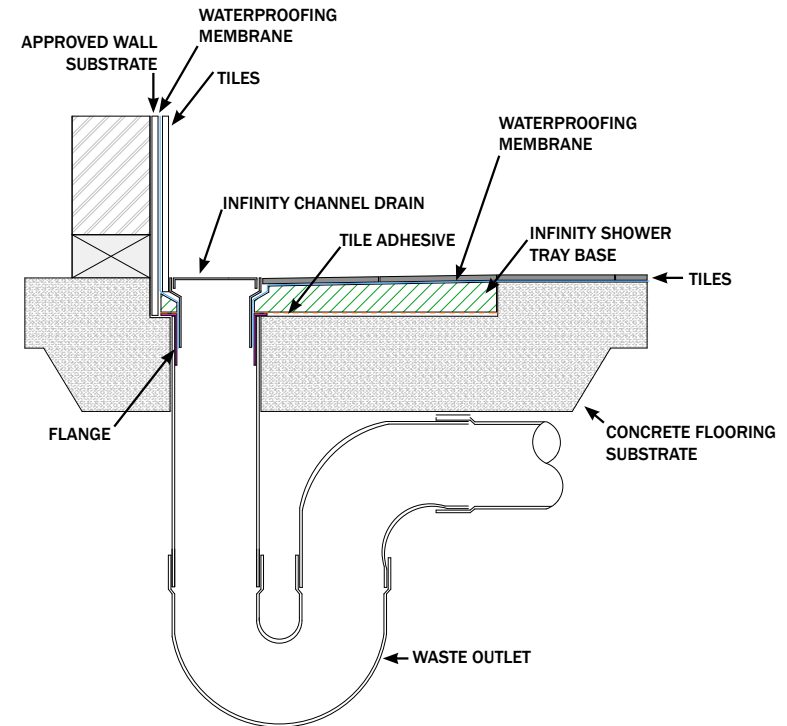
LEVEL ENTRY SHOWER TRAY
