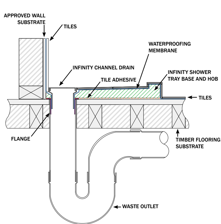
HOBBED SHOWER TRAY
