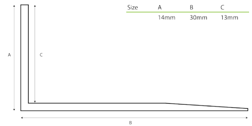
Alum Max-Finish Waterstop Concealed 2.5m
